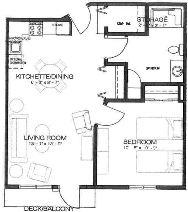
Type A - Floors 3 & 4
