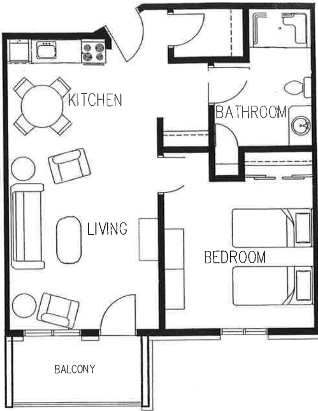
Type A - Floors 1 & 2
